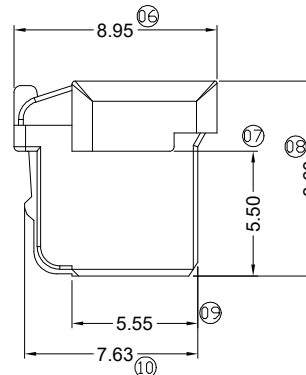
2*04P~2*09P Shape Scale 1:1
